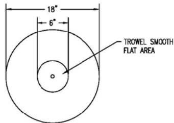
2 BOTTOM VIEW
