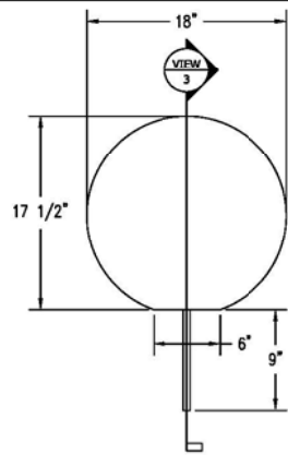
1 TOP VIEW
