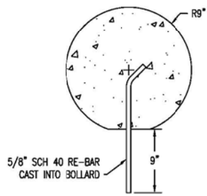
3 SECTION VIEW
